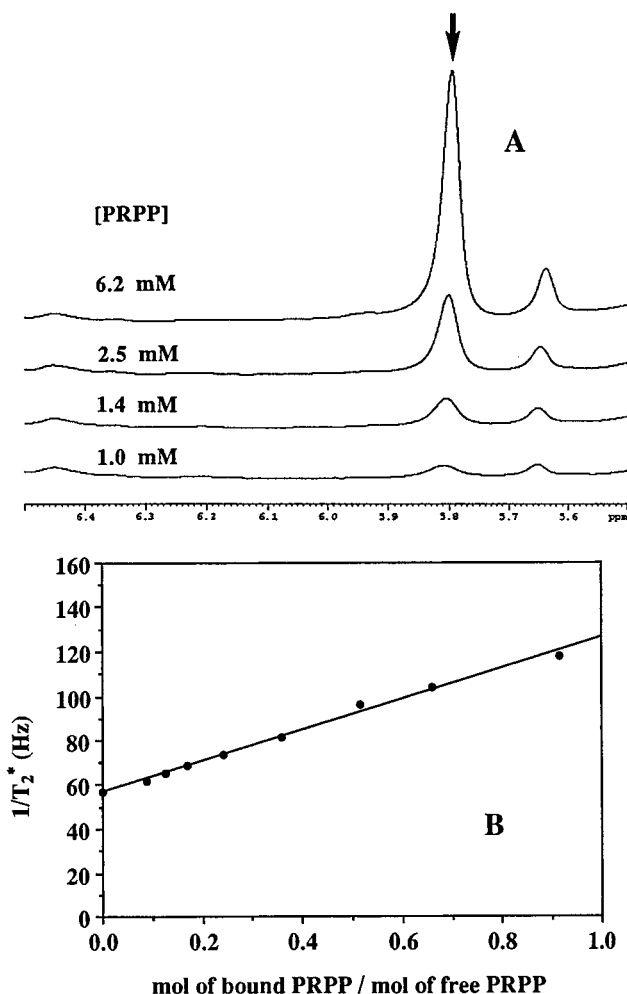
FIGURE 5: 1 H NMR PRPP titration of 0.5 mM OPRTase. (A) C1H proton resonance of unbound PRPP is at 5.8 ppm (arrow). The C1H signal of enzyme-bound PRPP (6.2 ppm) was identified using saturation transfer as described in Experimental Procedures. (B) A linear least-squares plot of 1/T_2^* versus bound/free PRPP in the titration of WT OPRTase by PRPP. The values of 1/T_2^* were determined by measuring the linewidths of free PRPP C1 proton resonance. The ratios of bound/free PRPP were calculated on the basis of the known dissociation constant for PRPP (27). The slope of the line ( 69\text{ s}^{-1} ) represents the dissociation rate constant of PRPP.
