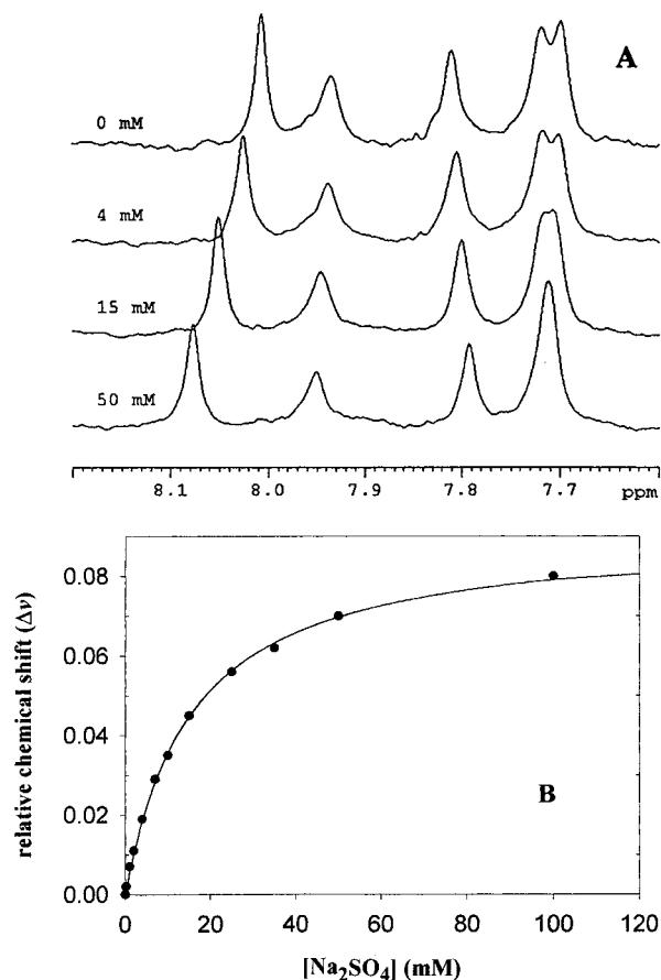
FIGURE 7: (A) Titration of histidine C2 proton resonances of 540 \mu\text{M} WT OPRTase by Na 2 SO 4 , showing fast exchange. The His-105 C2 proton at 8.02 ppm shifts progressively downfield as the Na 2 SO 4 concentration increases (0–50 mM). A lower limit for the off-rate of sulfate ( 2400\text{ s}^{-1} ) was estimated on the basis of chemical shift changes. (B) A plot of His-105 C2 proton chemical shift changes versus total sulfate concentration. The curve represents a best fit by nonlinear least-squares regression using the equation \Delta\nu = \nu_{\text{max}}(L_T/K_D + L_T) , where \nu_{\text{max}} is the maximal chemical shift change at saturating Na 2 SO 4 concentration, and L_T , or free Na 2 SO 4 concentration, is given by L_T = 0.5((K_D + E_T + L_T) - ((K_D + E_T + L_T)^2 - 4E_T L_T)^{1/2}) . E_T and L_T are total enzyme and Na 2 SO 4 concentrations, respectively. The K_D value derived from the best fit curve was 15.2 mM.
